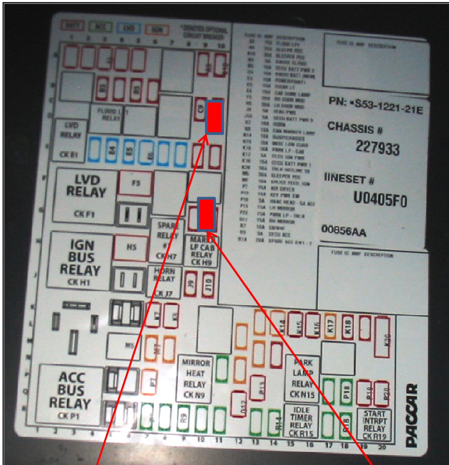
12v Power 10 Amp fuse Figure 3
